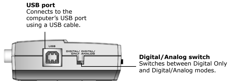
Figure 1-3: Jacks, connectors and ports on Sound Blaster
