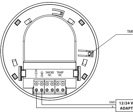
Diagram 1 - DC Power adapter connection.
