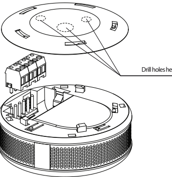
Fig. 2 - Constant current or alarm system hub connecting terminals installation.
