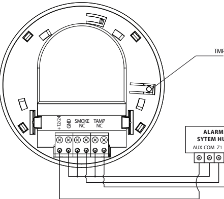
Diagram 2 - Alarm system hub connection.
