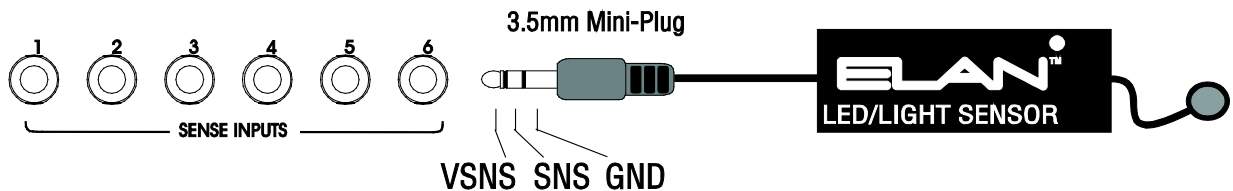
Figure 3-6: Sense Inputs
