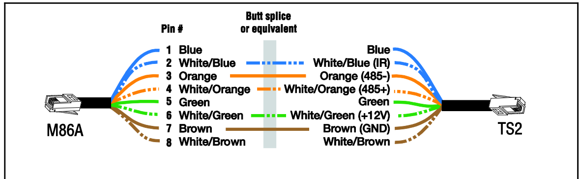
Figure 3-4: Wiring Configuration
