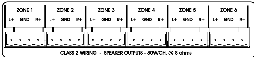
Figure 3-9: Speaker Connections
