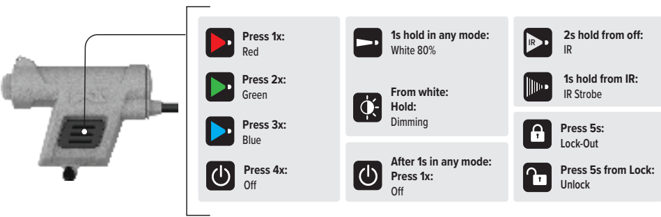
Figure 2 – Switch Operation
