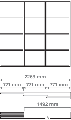
Combination with 3 doors and the 3-track rail. 3× 771 mm doors
