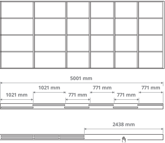
Combination with 6 doors and the 2-track rail. 4× 771 mm and 2× 1021 mm doors
