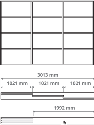
Combination with 3 doors and the 3-track rail. 3× 1021 mm doors
