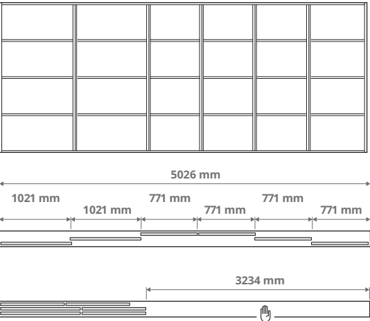
Combination with 6 doors and the 3-track rail. 4× 771 mm and 2× 1021 mm doors
