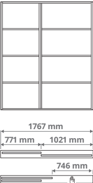
Combination with 2 doors and the 2-track rail 1× 771 mm and 1× 1021 mm door
