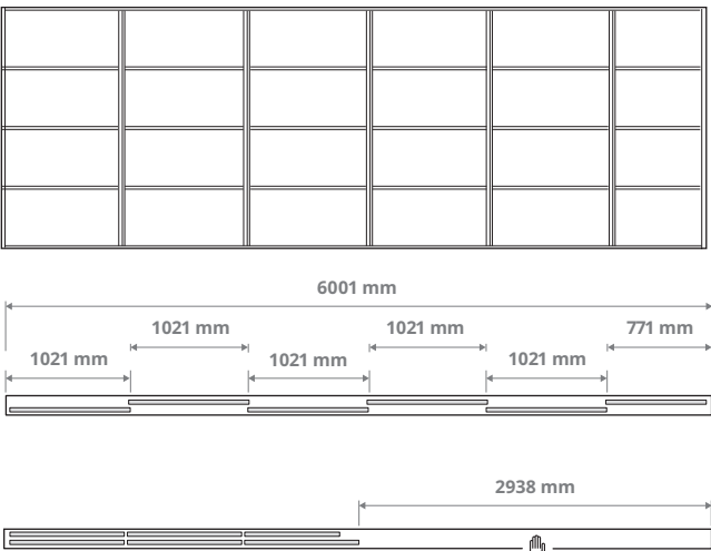
Combination with 6 doors and the 2-track rail. 5× 1021 mm and 1× 771 mm doors
