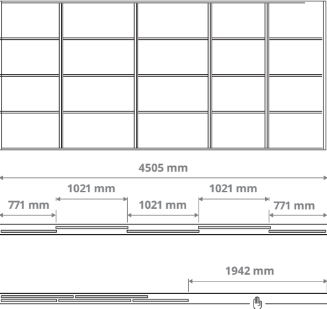
Combination with 5 doors and the 2-track rail. 2× 771 mm and 3× 1021 mm doors
