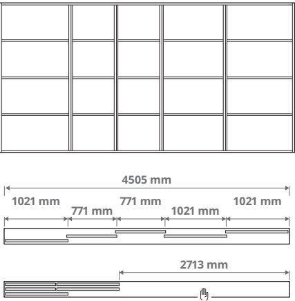
Combination with 5 doors and the 3-track rail. 2× 771 mm and 3× 1021 mm doors
