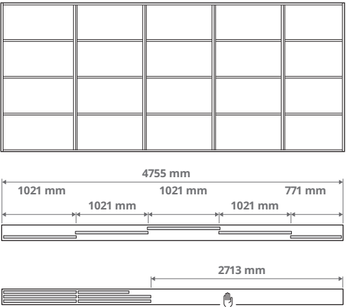
Combination with 5 doors and the 3-track rail. 1× 771 mm and 4× 1021 mm doors
