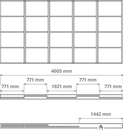
Combination with 5 doors and the 2-track rail. 4× 771 mm and 1× 1021 mm doors
