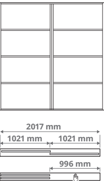
Combination with 2 doors and the 2-track rail 2× 1021 mm doors
