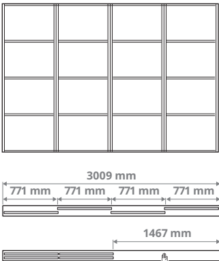
Combination with 4 doors and the 2-track rail 4× 771 mm doors
