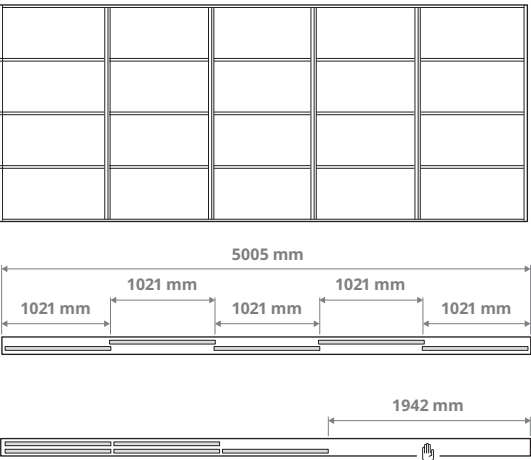
Combination with 5 doors and the 2-track rail. 5× 1021 mm doors
