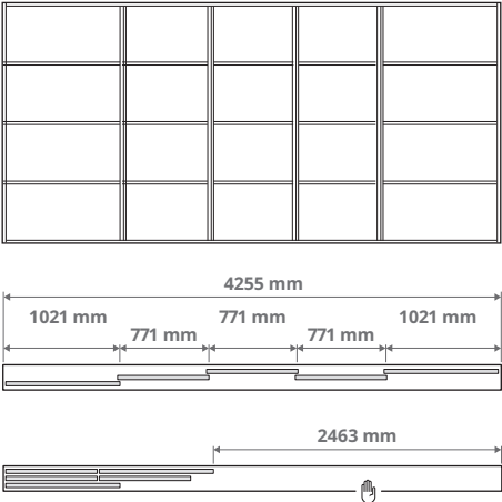
Combination with 5 doors and the 3-track rail. 3× 771 mm and 2× 1021 mm doors
