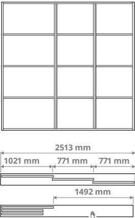
Combination with 3 doors and the 3-track rail. 2× 771 mm and 1× 1021 mm doors
