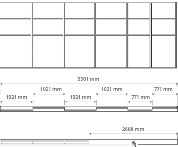
Combination with 6 doors and the 2-track rail. 4× 1021 mm and 2× 771 mm doors
