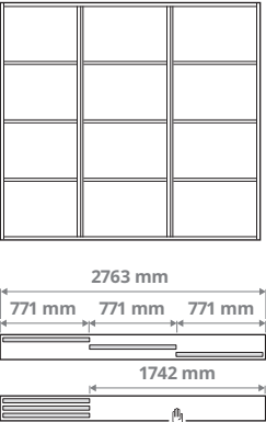
Combination with 3 doors and the 3-track rail. 1× 771 mm and 2× 1021 mm doors
