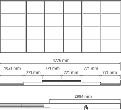
Combination with 6 doors and the 3-track rail. 5× 771 mm and 1× 1021 mm
