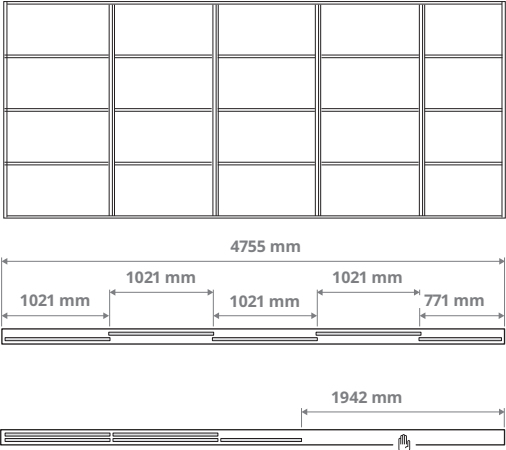
Combination with 5 doors and the 2-track rail. 1× 771 mm and 4× 1021 mm doors
