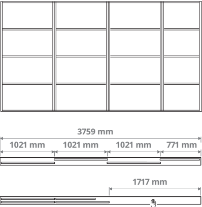
Combination with 4 doors and the 2-track rail. 1× 771 mm and 3× 1021 mm doors
