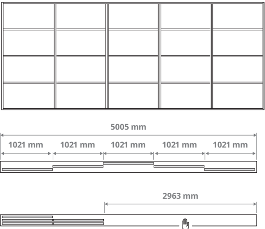
Combination with 5 doors and the 3-track rail. 5× 771 mm
