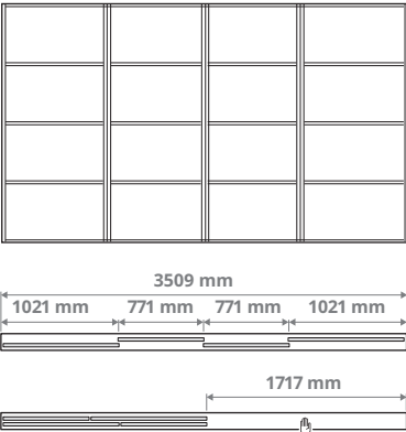
Combination with 4 doors and the 2-track rail. 2× 771 mm and 2× 1021 mm doors
