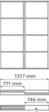
Combination with 2 doors and the 2-track rail 2× 771 mm doors
