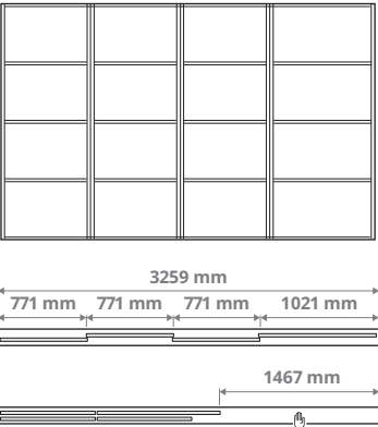
Combination with 4 doors and the 2-track rail 3× 771 mm and 1× 1021 mm doors
