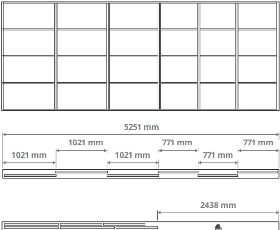
Combination with 6 doors and the 2-track rail. 3× 771 mm and 3× 1021 mm doors
