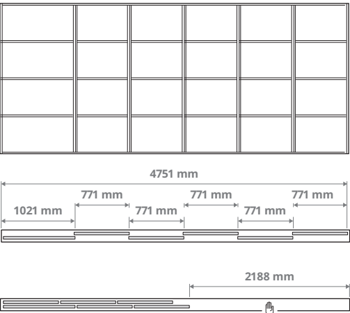
Combination with 6 doors and the 2-track rail. 5× 771 mm and 1× 1021 mm doors
