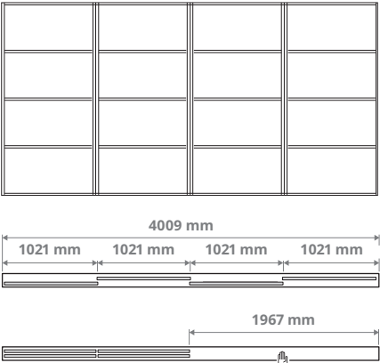
Combination with 4 doors and the 2-track rail. 4× 1021 mm doors
