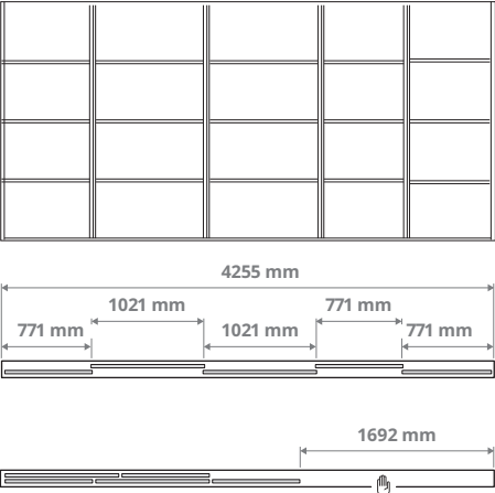
Combination with 5 doors and the 2-track rail. 3× 771 mm and 2× 1021 mm doors
