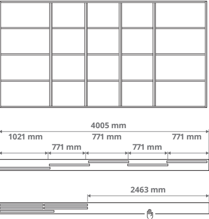
Combination with 5 doors and the 3-track rail. 4× 771 mm and 1× 1021 mm doors
