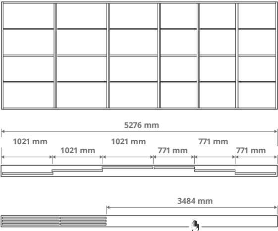
Combination with 6 doors and the 3-track rail. 3× 771 mm and 3× 1021 mm doors
