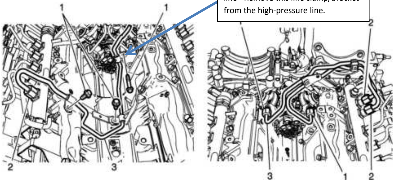
Fig. 8: High and low fuel pressure line removal
