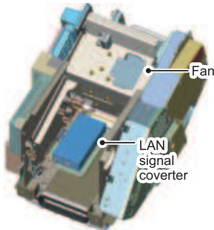
RTR-107 rear-view
