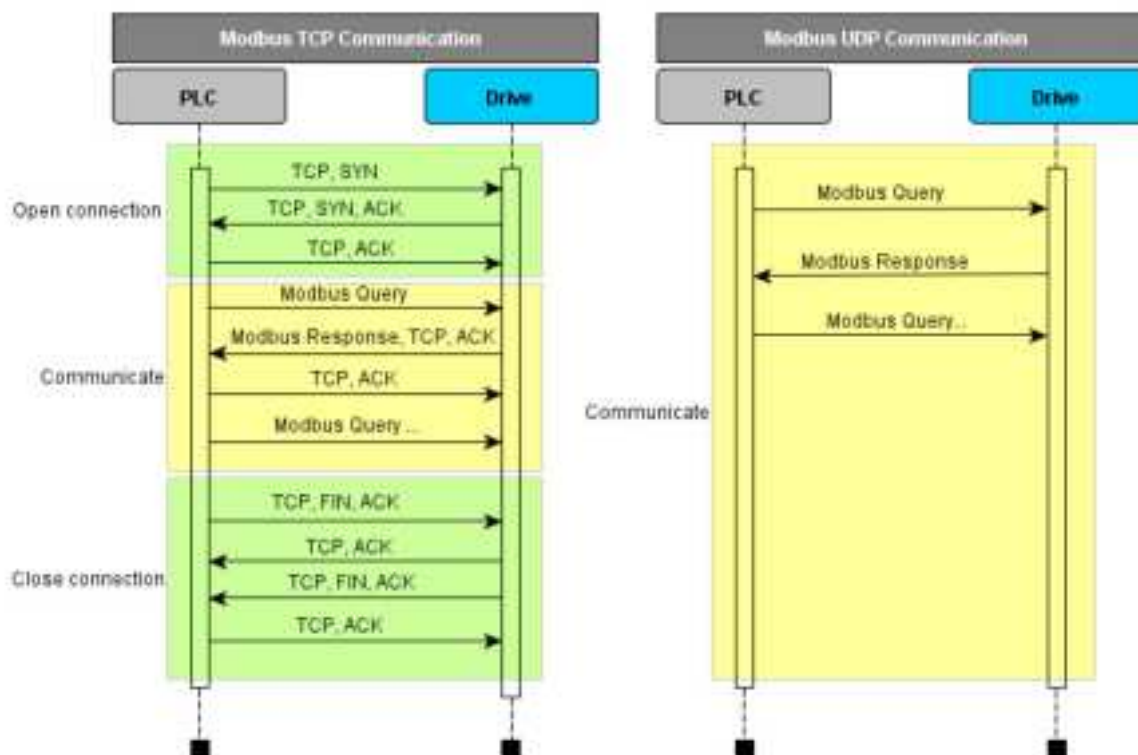
Figure 6-7. Modbus TCP and UDP communication comparison
