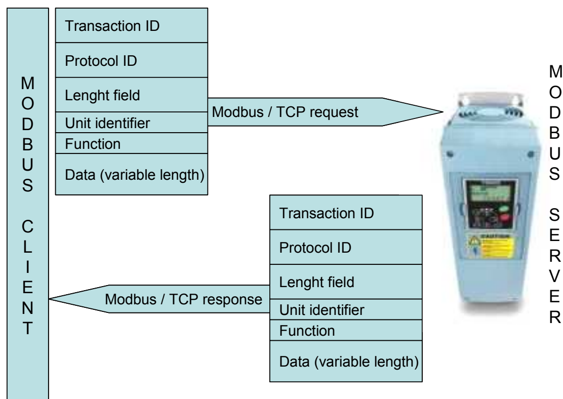
Figure 5-1: Modbus Transaction
