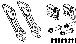
500205943 Servosaver-Unit Servosaver-Einheit
