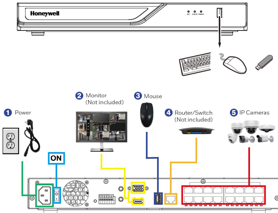
Figure 2-1 Devices Connection
