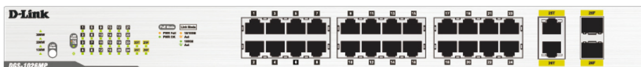
Figure 3 – DGS-1026MP Front panel LEDs
