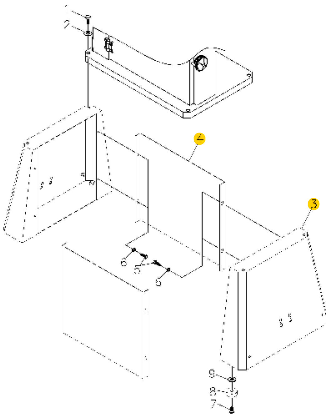
Stand Assembly
