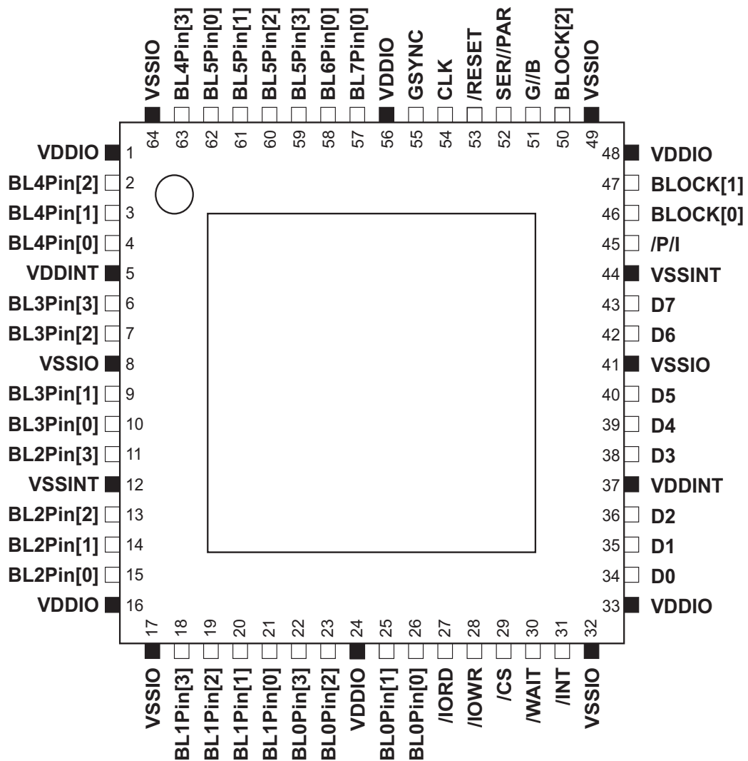
Figure 1-1. Parallel Pinout
