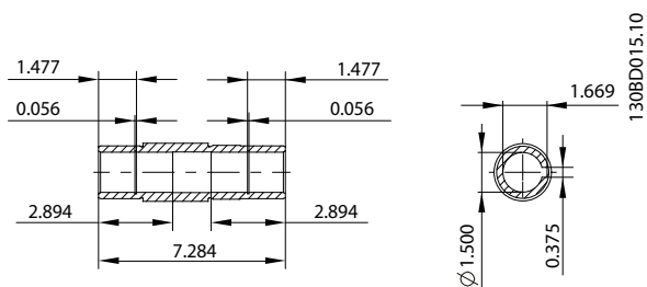
Figure 4.4 1 1/2 inch shaft
