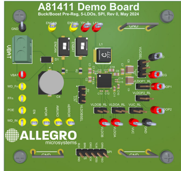
Figure 1: A81411 Evaluation Board
