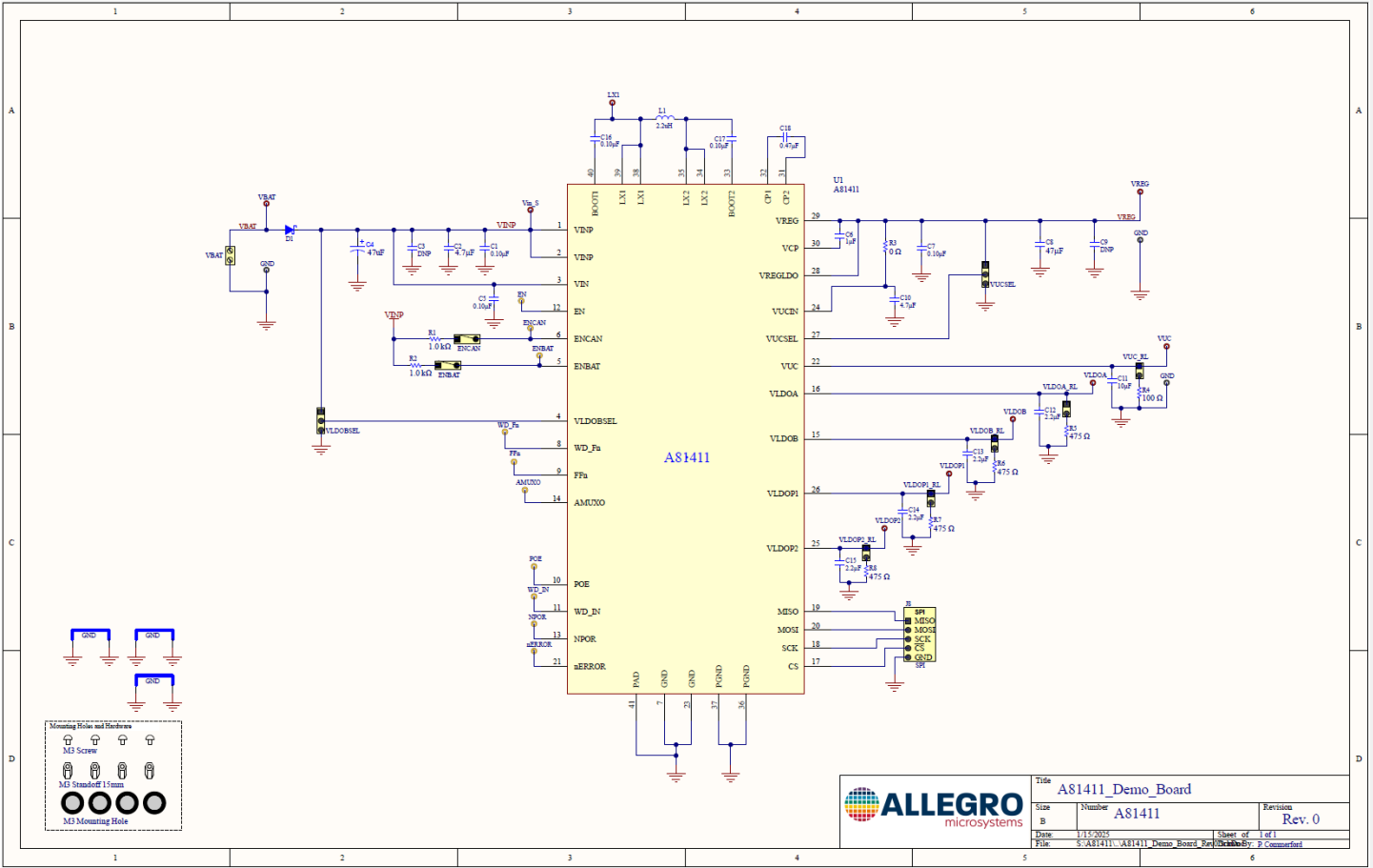
Figure 5: A81411 evaluation board schematic
