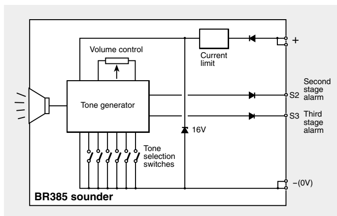
Fig 1 Simplified block diagram
