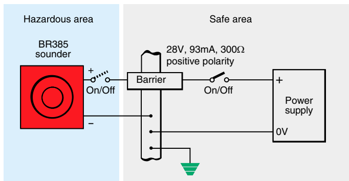
Fig 2 Single stage alarm using channel barrier
