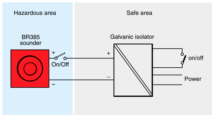
Fig 5 Single stage alarm using galvanic isolator
