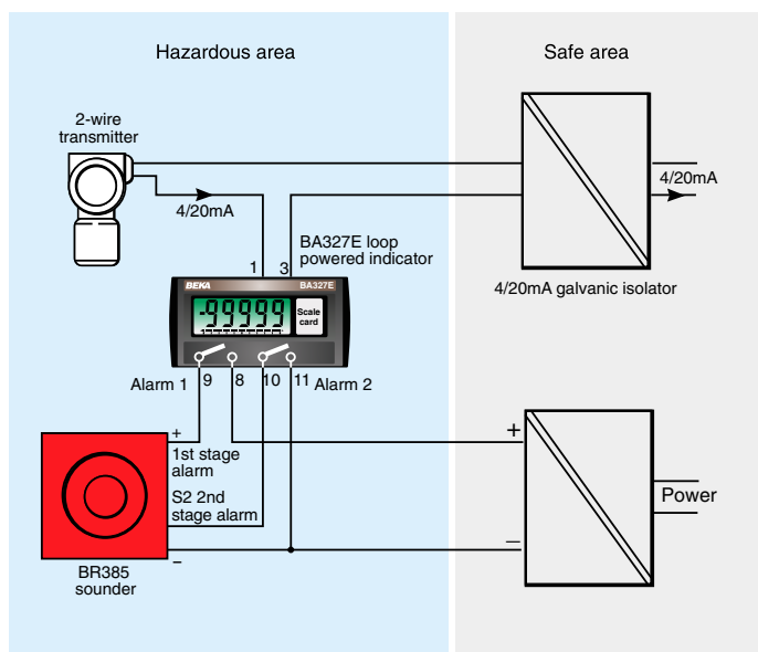
Fig 6 Loop-powered BA327E intrinsically safe indicator controlling BR385 first and second stage alarms.
