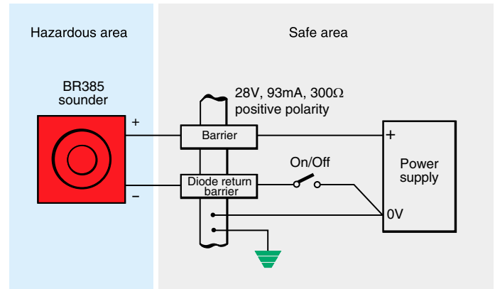
Fig 3 Single stage alarm using two channel barrier
