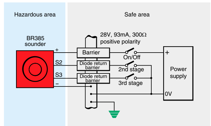
Fig 4 Multi-stage alarm using Zener barrier
