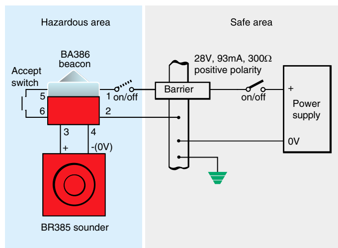
Fig 7 Combined circuit for BR385 sounder and BA386 beacon
