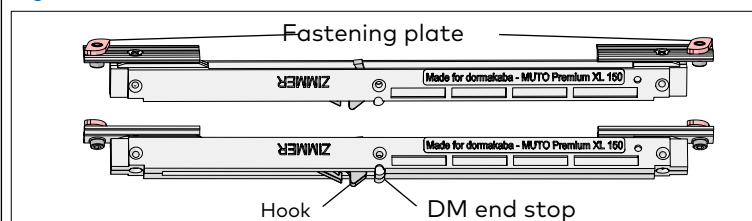
Fig. 14.10 LH DM unit fastening plates rotated
