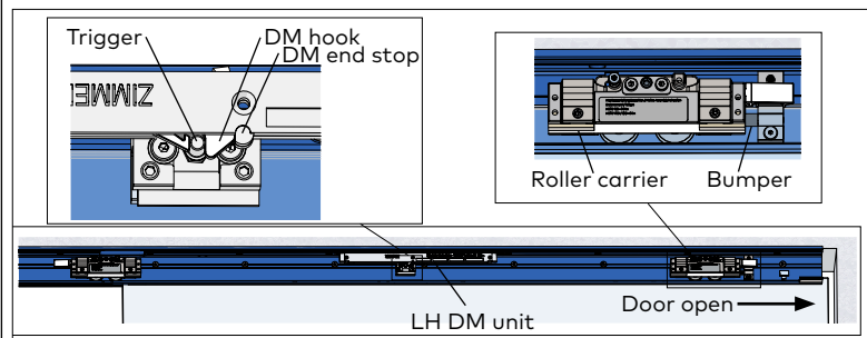
Fig. 14.12 DM unit hook positioned in trigger
