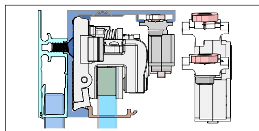
Fig. 14.15 LH DM unit aligned in track
