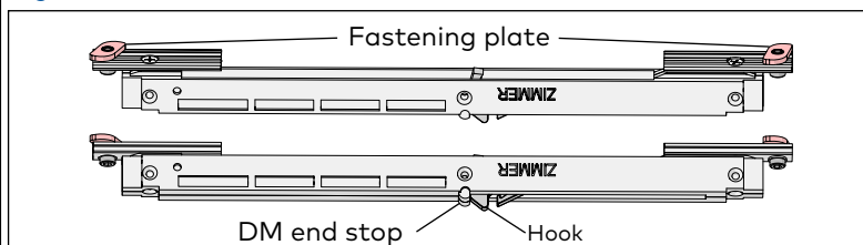
Fig. 14.2 RH DM unit fastening plates rotated
