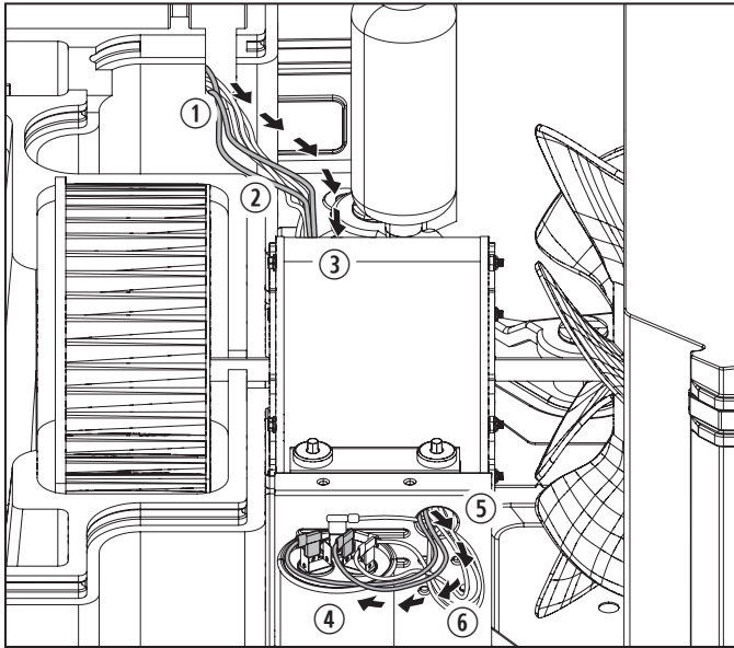
31 Routing wires through the fan motor mount to the capacitor
