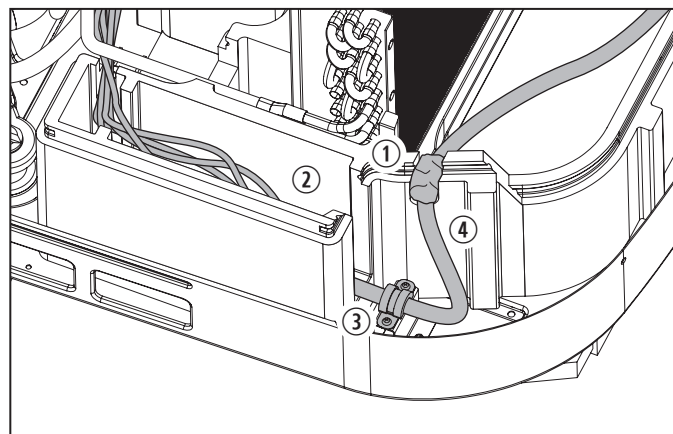
30 Securing the strain relief
