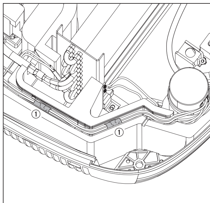
82 Putty location and placement
