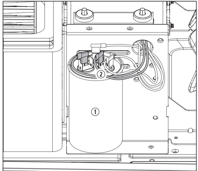
26 Disconnecting the compressor wires from the capacitor
