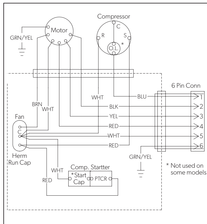
14 Blizzard NXT AC unit wiring diagram
