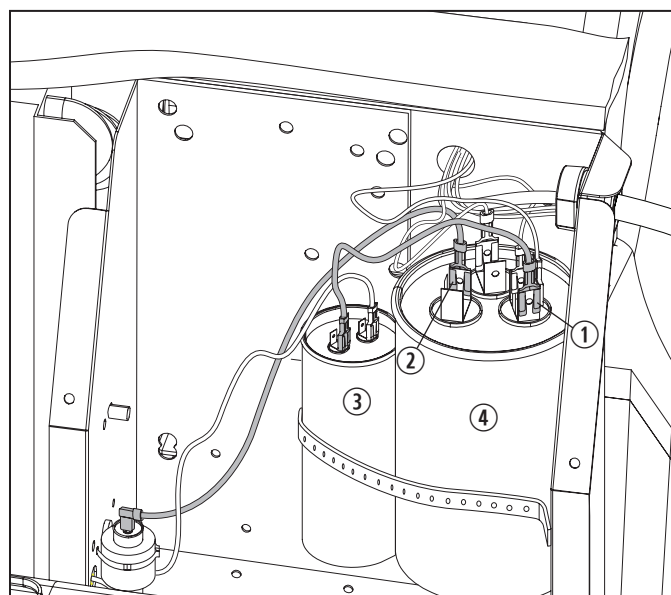
59 Disconnecting the start capacitor
