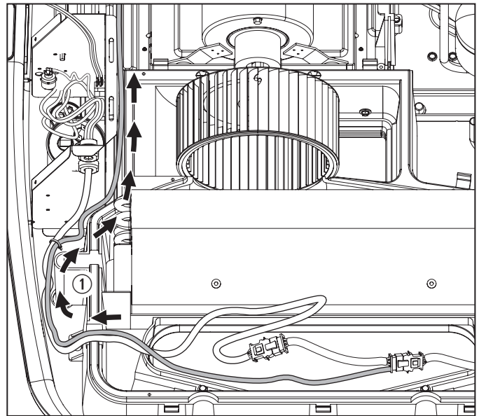
55 Routing the blue wire
