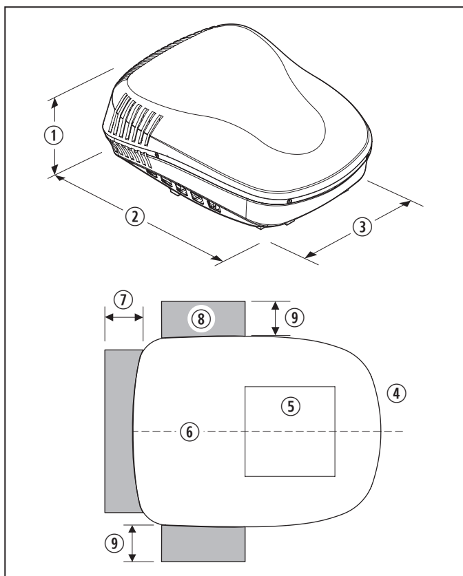
3 Blizzard NXT AC unit shroud dimensions
