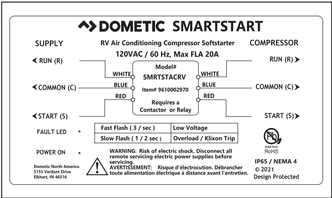
11 Device data plate
