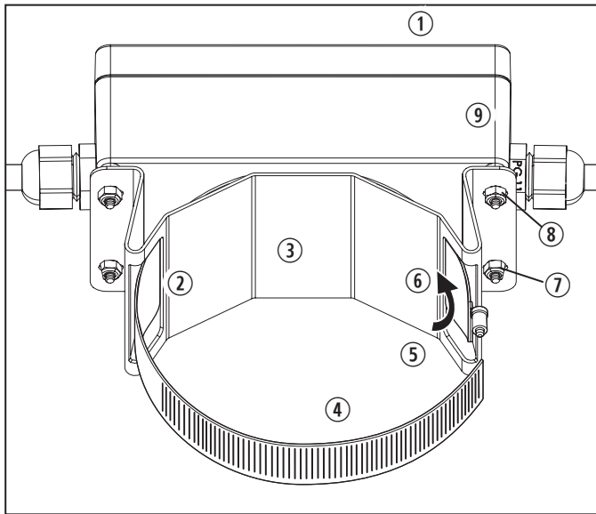
23 Attaching the hose clamp (supply side on the right)
