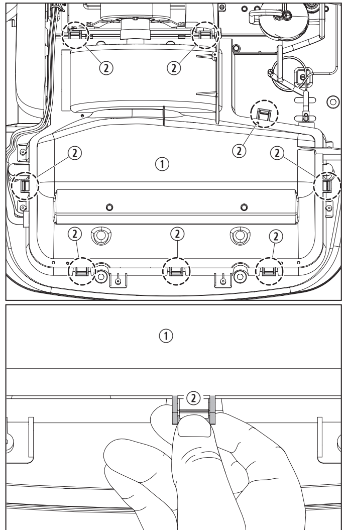
66 Reinstalling the evaporator shroud
