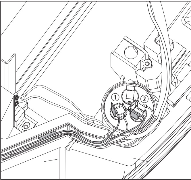
91 Attaching the device supply harness wires
