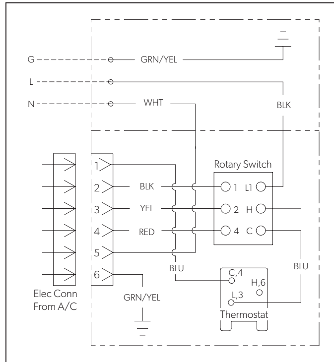
15 ADB wiring diagram - All AC unit models
