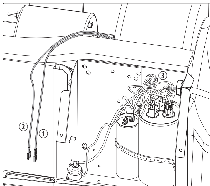
58 Pulling the compressor wires
