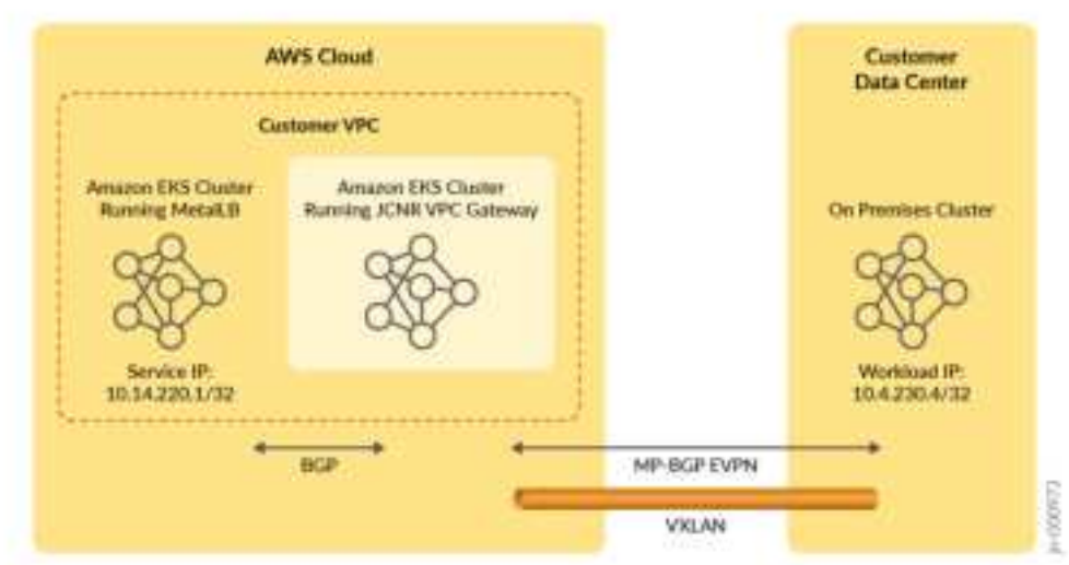
Figure 5: Cloud-Native Router VPC Gateway
