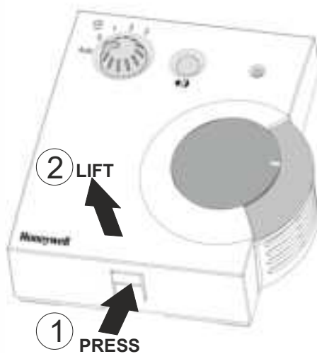
Fig. 1. Cover disassembly
