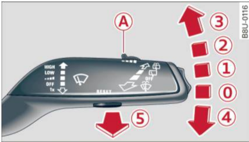
Fig. 39 Windshield wiper lever
