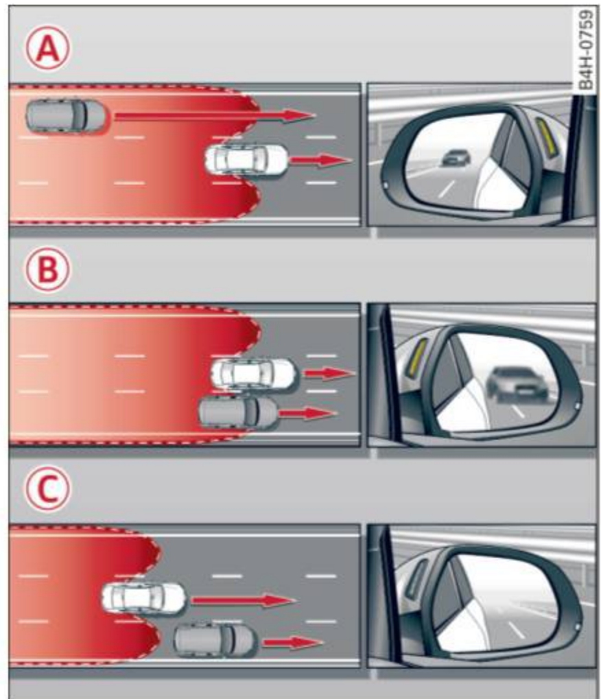
Fig. 81 Driving situations
