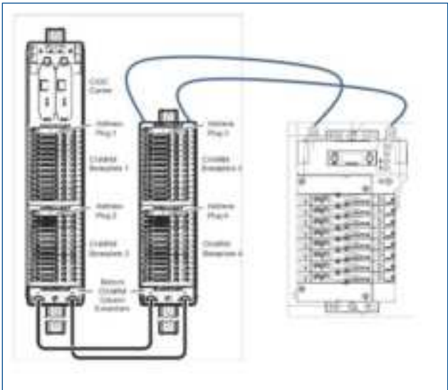
Connection to DeltaV Electronic Marshalling.
