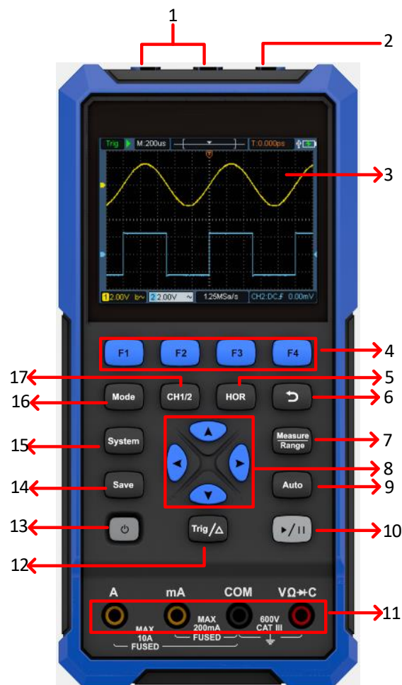
Figure 4: Front Panel of the Oscilloscope
