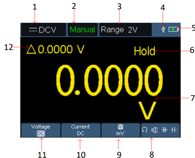
Multimeter Interface
