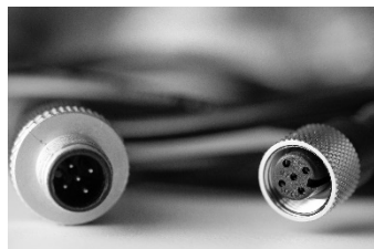
M12 Connector
