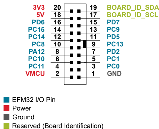
Figure 4.2. EXP Header
