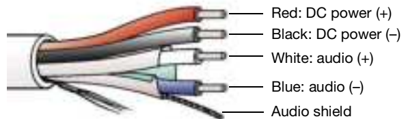
Belden 1502 Composite Cable
