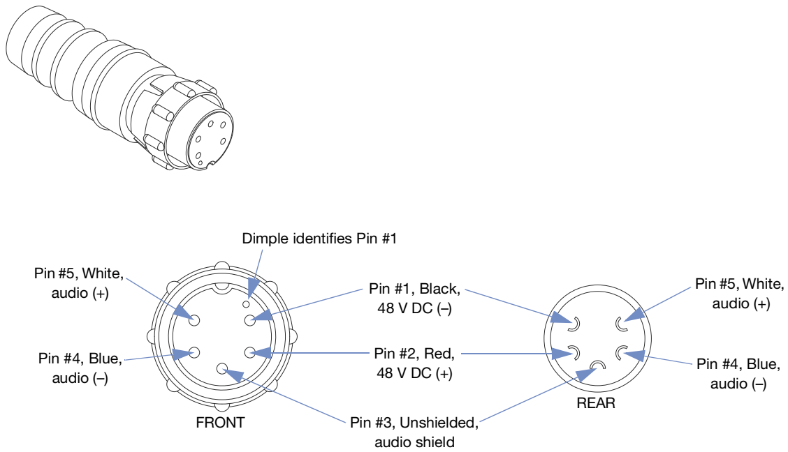
Pin Destinations for EN3 5-Pin Female Cable Mount Connector
