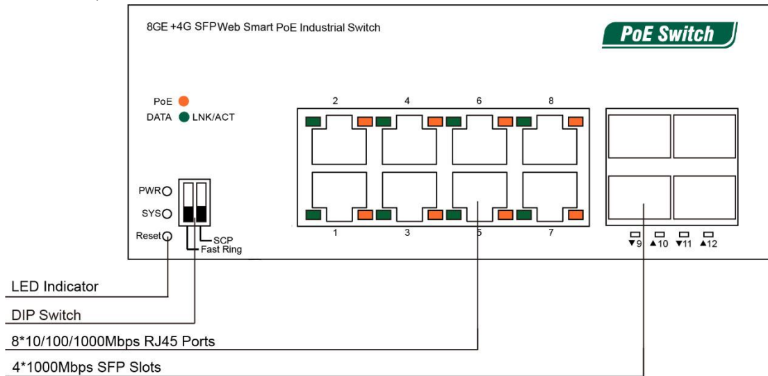
Figure 3-1 Front panel of the 8GE +4G SFP Switch
