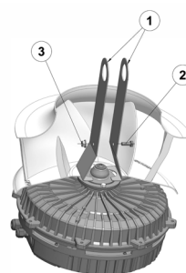
1. Lifting aid – 2. Locking screw – 3. Lock nut
