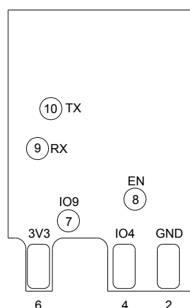
Pin Layout (Bottom View)
