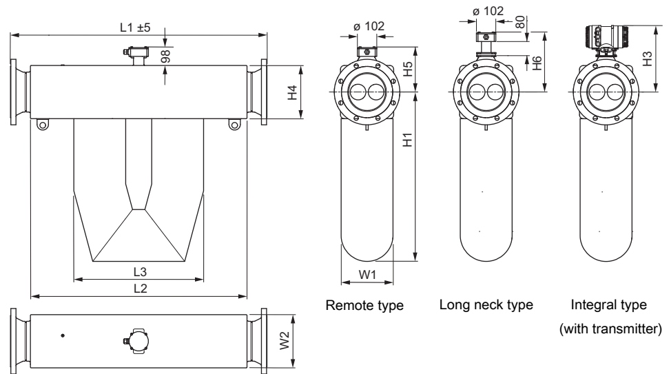
Fig. 22: Dimensions in mm
