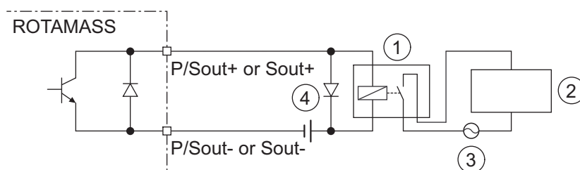
Fig. 37: Passive status output connection P/Sout for solenoid valve circuit
