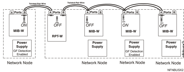
Figure 3.15 Bus (EXAMPLE 2)
