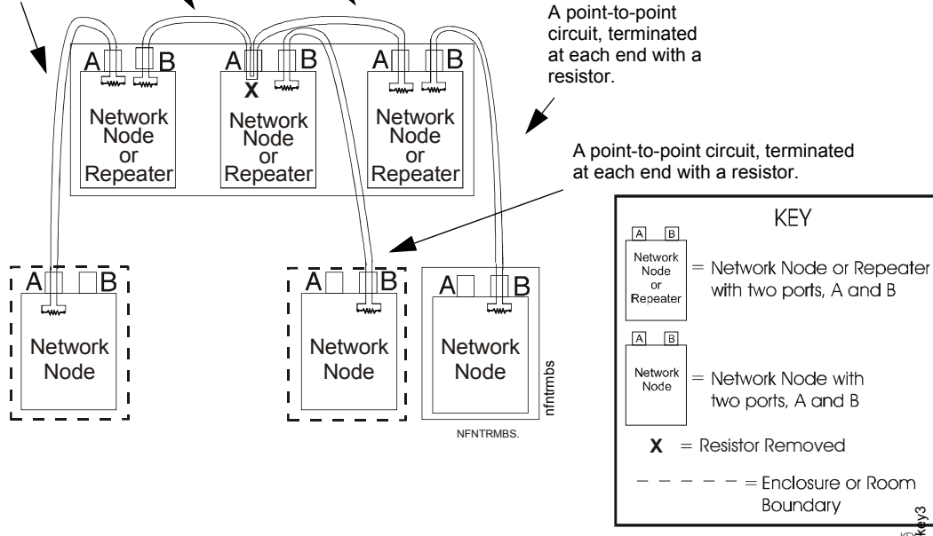
Figure 3.8 Bus Termination
