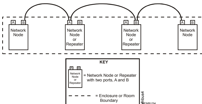
Figure 3.5 Bus Configuration (NFPA Style 4 Only)
