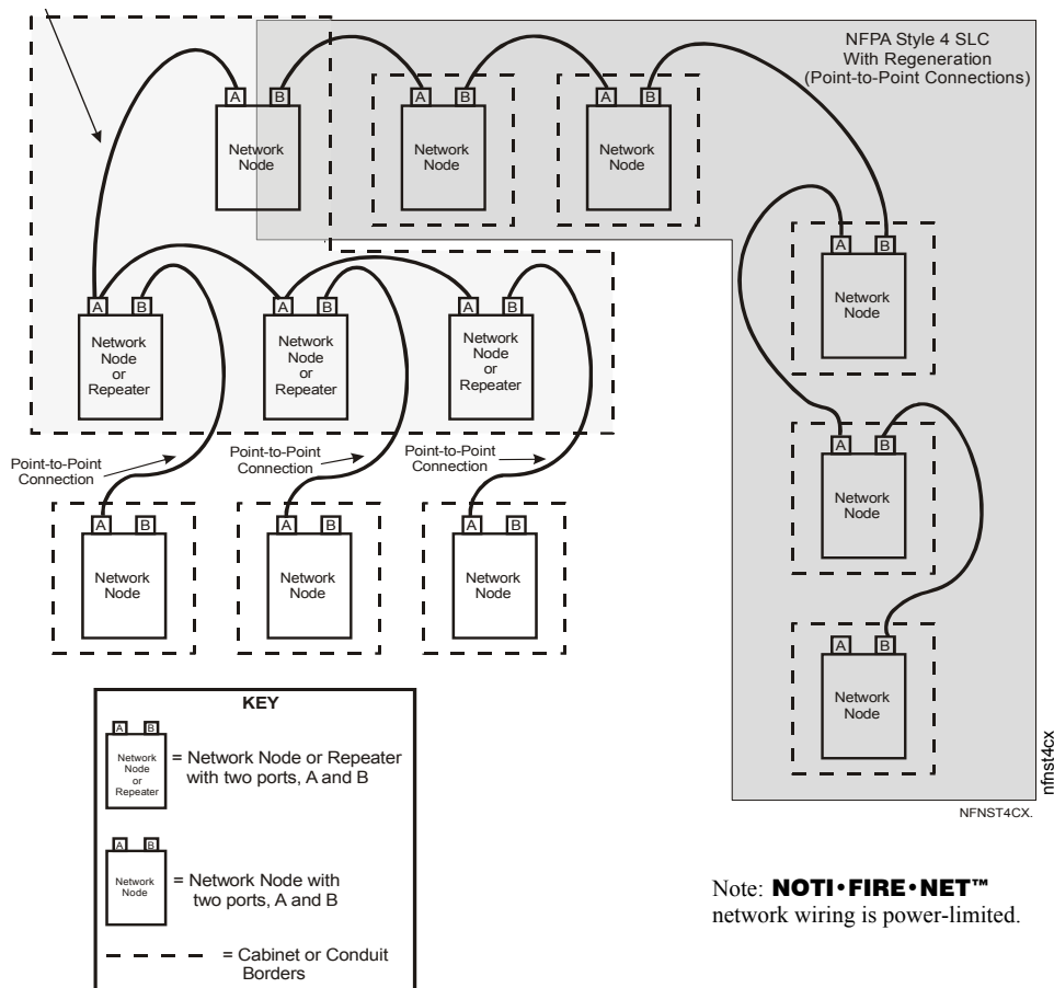
Figure 3.1 Style 4 Configurations
