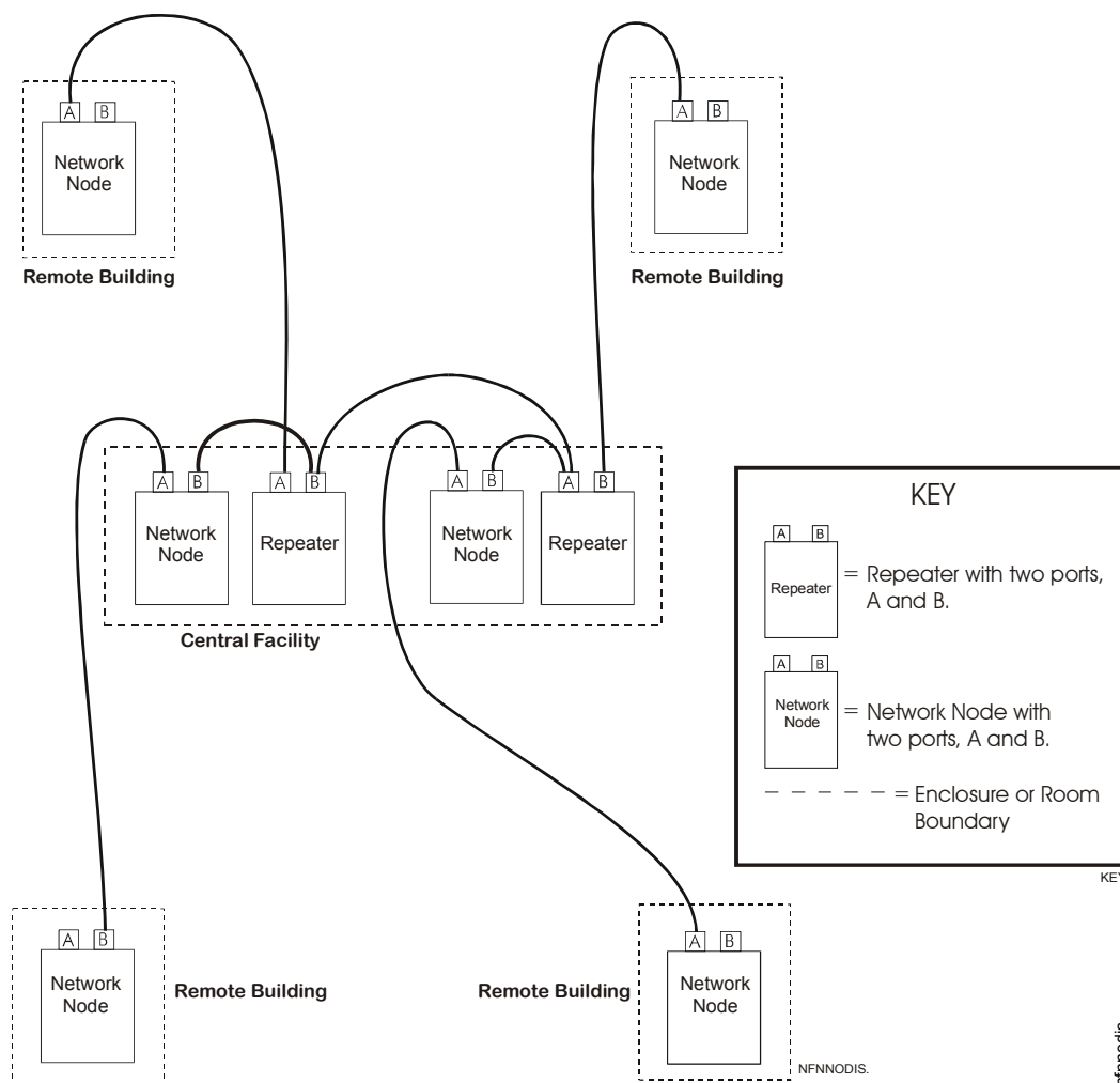
Figure 3.6 Combination Wiring
