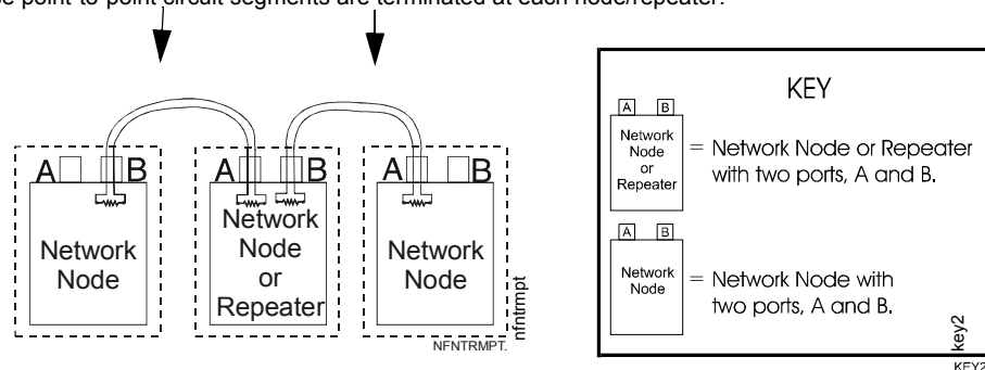
Figure 3.7 Point-to-Point Termination
