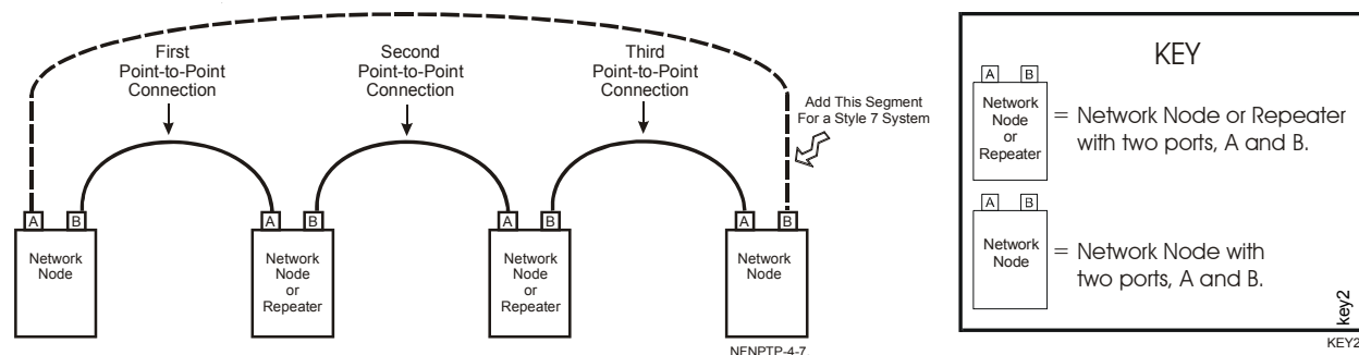
Figure 3.4 Point-to-Point Configuration for NFPA Style 4 or Style 7
