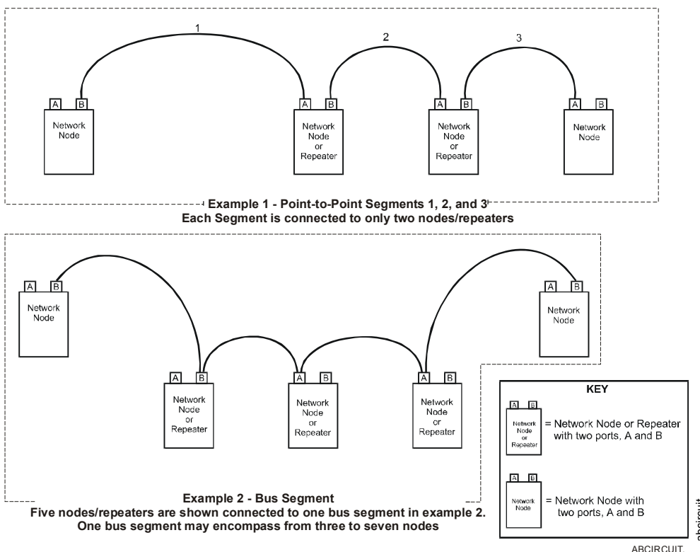
Figure 4.1 Circuit Wiring Layout
