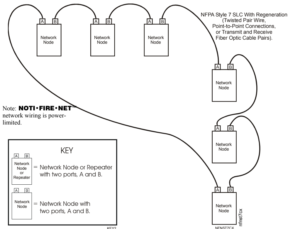
Figure 3.3 Style 7 Configurations
