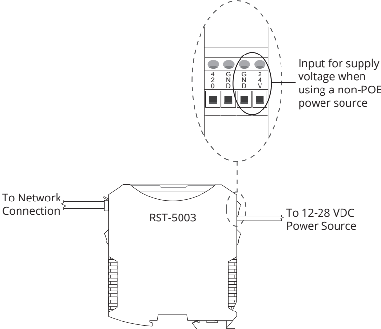
External 12-28VDC Power Supply Wiring
