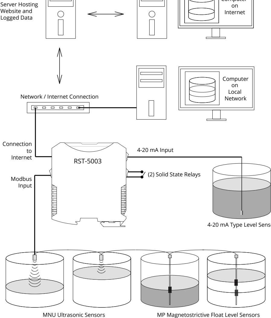
Modbus System & Network Diagram
