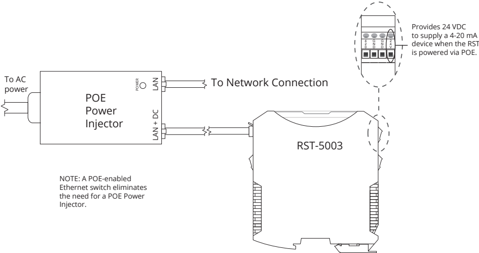
POE (Power Over Ethernet) Wiring
