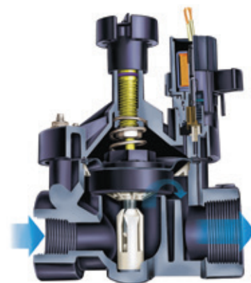
PESB Cutaway
