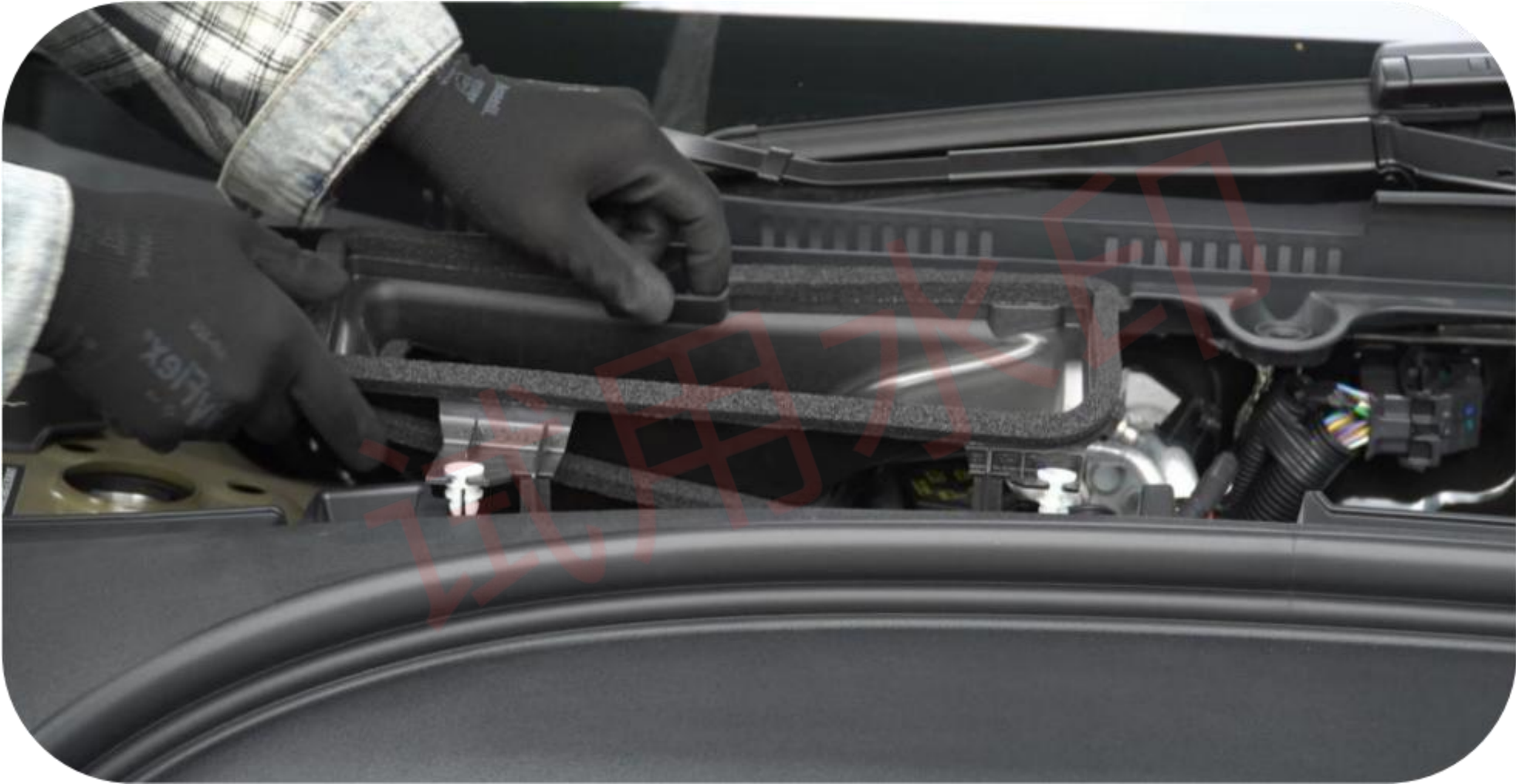
10. Remove the air inlet
