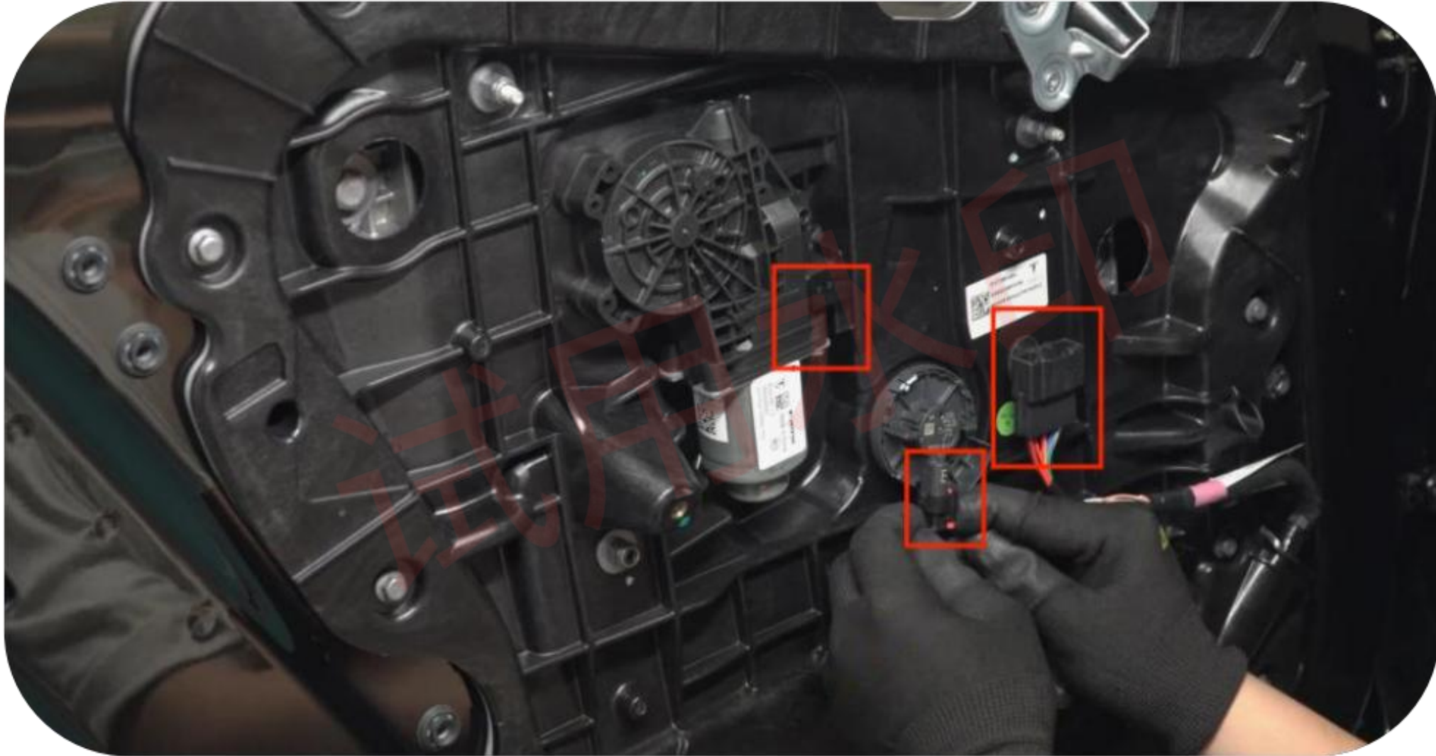
34. Pull out all the plugs and buckles on the waterproof panel
