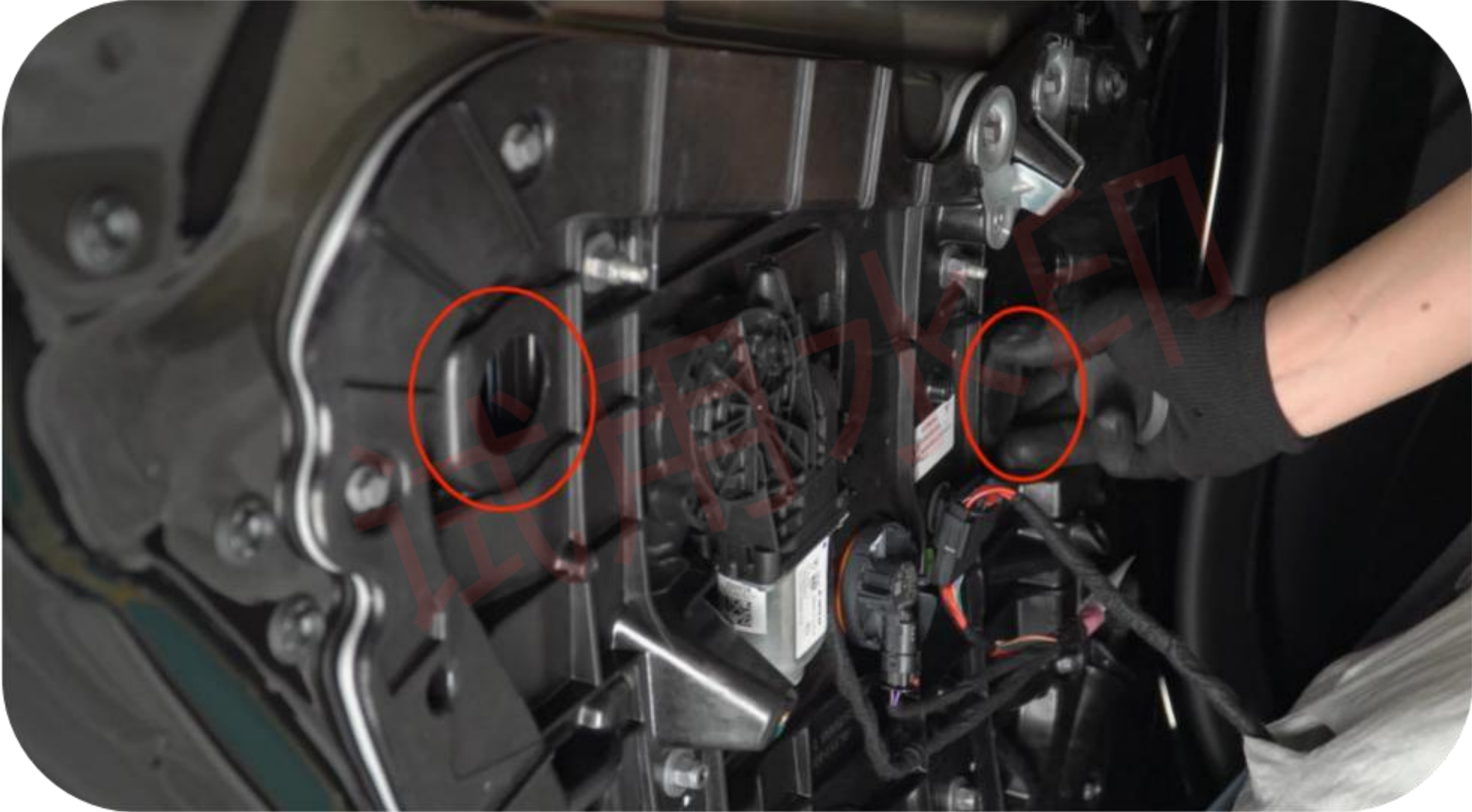
31. Remove the two rubber rings
