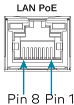
LAN PoE Pin Assignment
