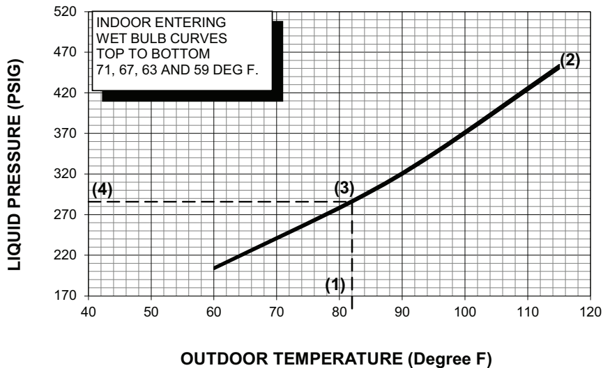
PRESSURE CURVES for 5A7A5018A1
