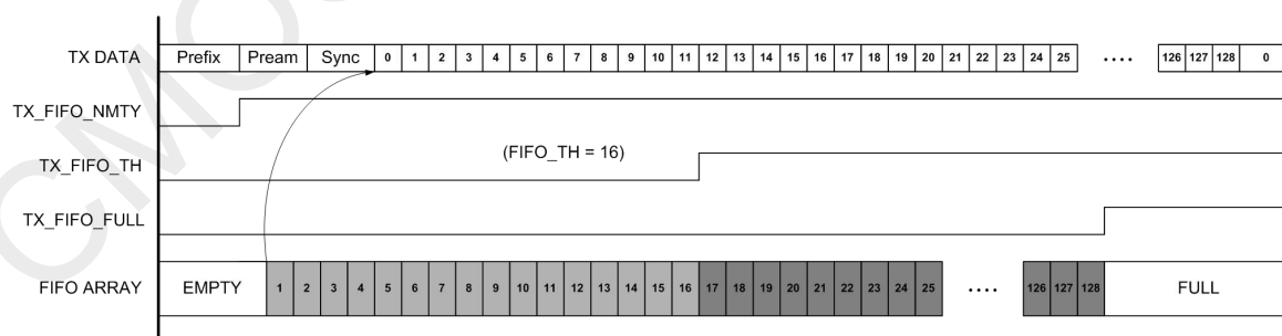
Figure 22. CMT 2310A TX FIFO Interrupt Timing
