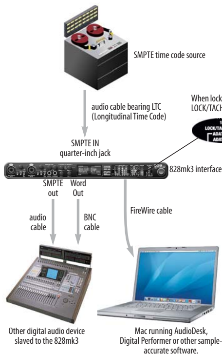
Figure 3-16: Connections for synchronizing the 828mk3 directly to SMPTE time code.
