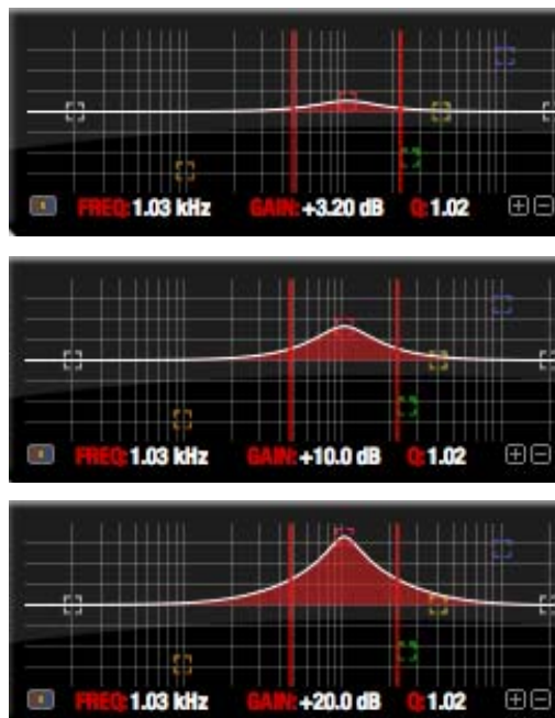
Figure 11-15: Type III EQ filter style.
