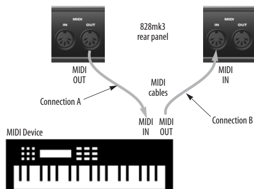
Figure 3-9: Connecting a MIDI device to the 828mk3.
