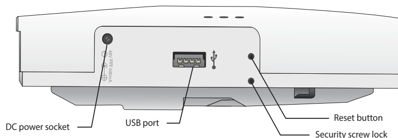
Figure 6 303H Series Side View
