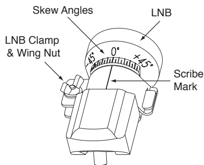
Figure 2-20 Skew Adjustment (European Systems Only)
