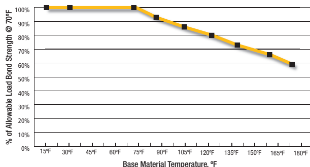
Load-Temperature Reduction Curve Concrete Base Materials
