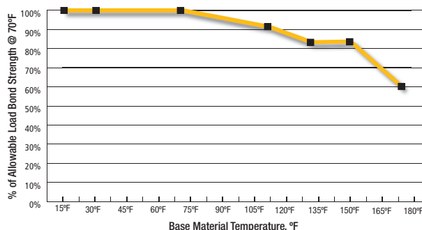
Load-Temperature Reduction Curve Masonry Units
