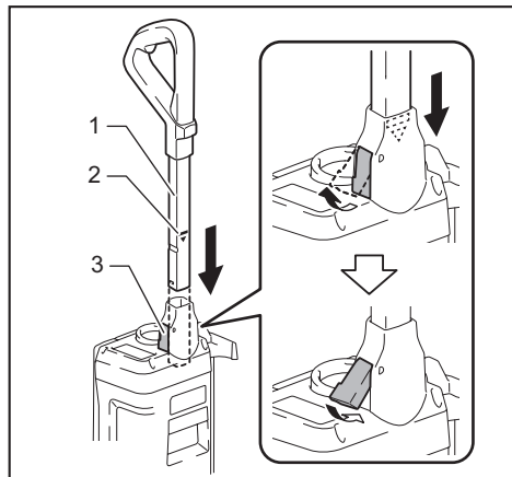
► 1. Handle pole 2. Red marking 3. Lock latch
