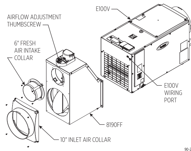
FIGURE 2 – ASSEMBLING AND MOUNTING THE 8190FF
