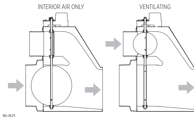
FIGURE 1 – DAMPER OPERATION
