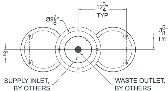
MOUNTING BASE DETAIL
