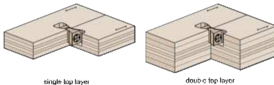
Fig 1.3 – HTC-P2P, single top layer vs double top layer CLT panels.
