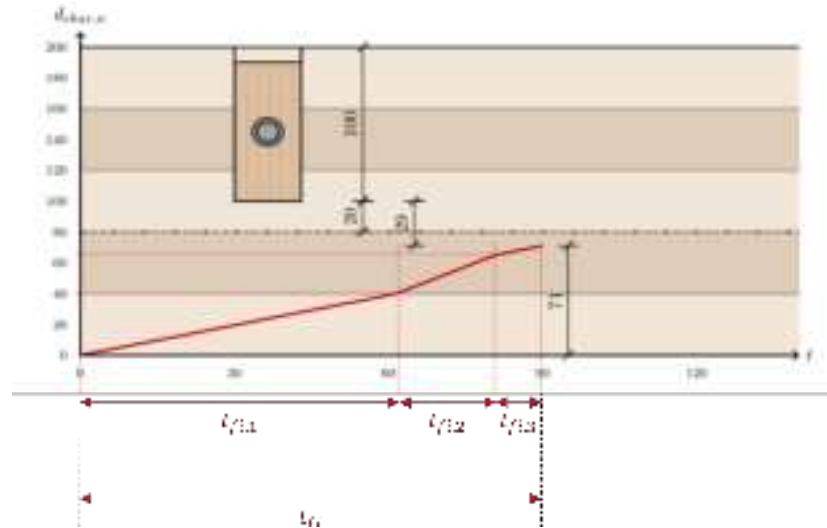
Fig 2.4 – Design example: calculation of the position of the char-line.
