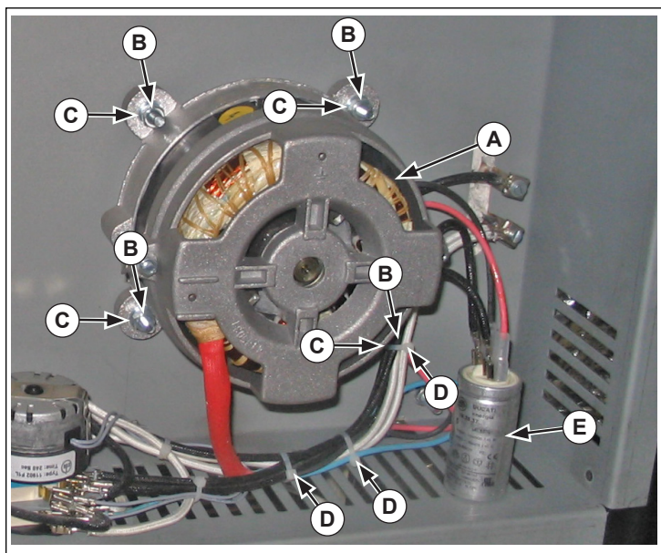
Figure 6. Motor, Hardware, Wires, Ties, Hardware and Capacitor
