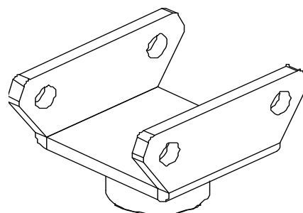
41 Fixing seat-upper
