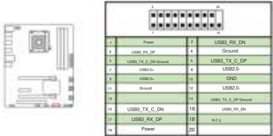
Figure 2-6 USB 3.0 interface
