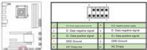
Figure 2-3 USB expansion port
