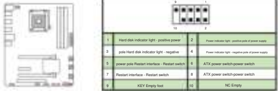
Figure 2-5 F_PANEL1 power-on interface
