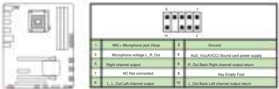
Figure 2-2 Front audio output
