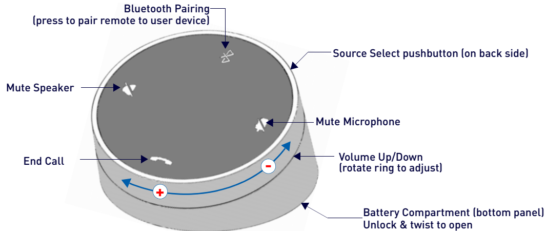
FIG. 4 Acendo Vibe Remote Control
