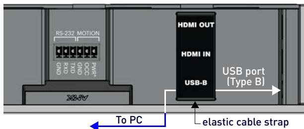
FIG. 29 Acendo Vibe Connector bay - Detail (ACV-5100 shown)
