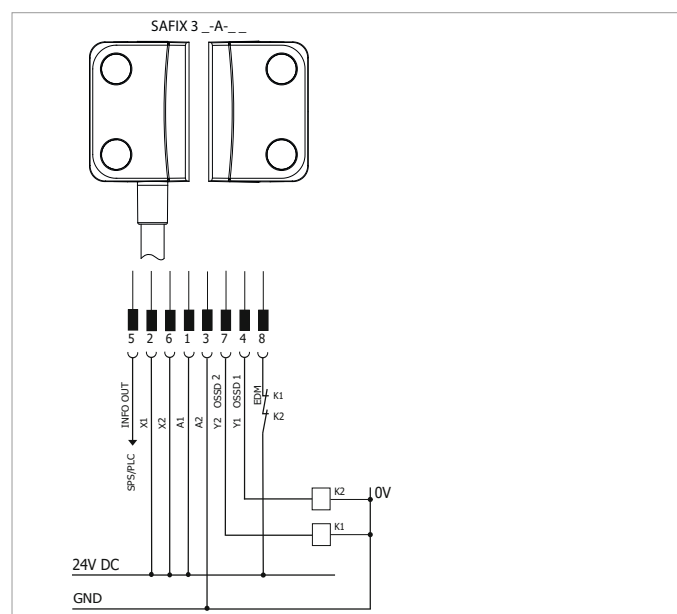
Figure 5: Connection with diagnosis output, automatic reset
