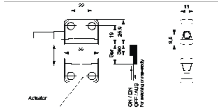
Figure 4: Switching distance
